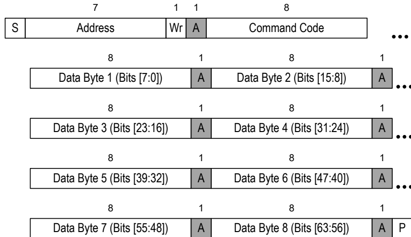
Figure 46: Write 64 Protocol
