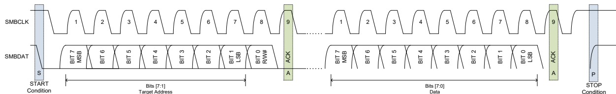
Figure 19: Data transfer over SMBus
