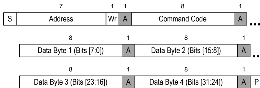
Figure 42: Write 32 Protocol
