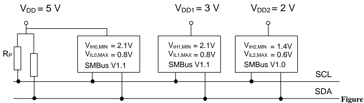
2.1: SMBus topology
