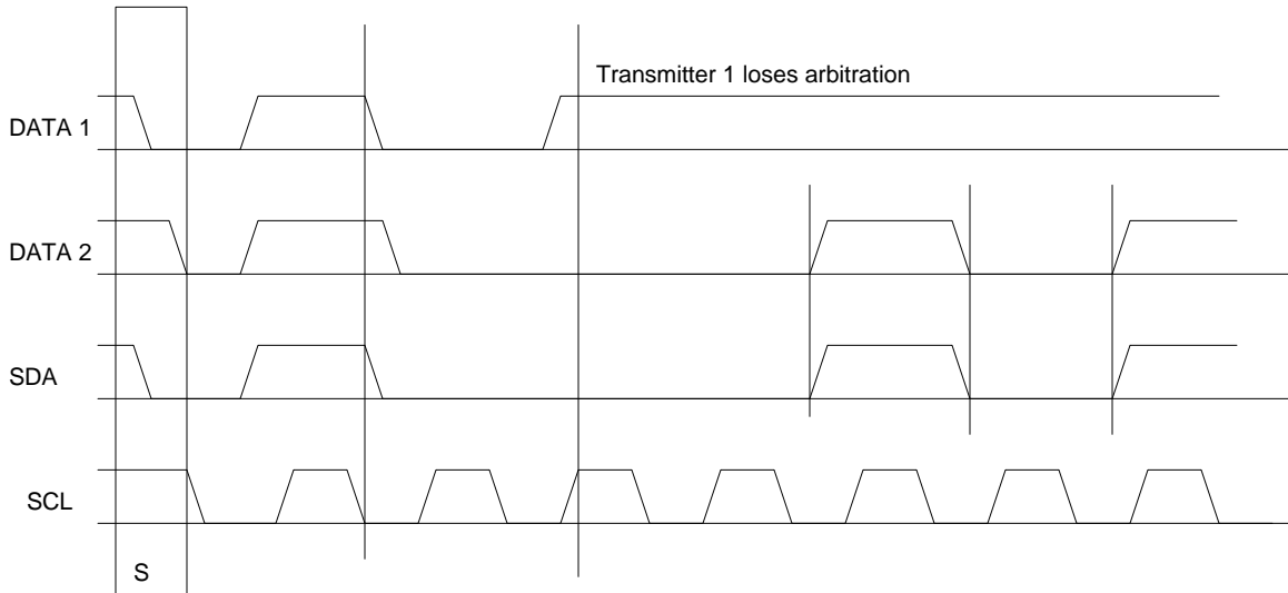
Figure 5.2: SMBus arbitration
