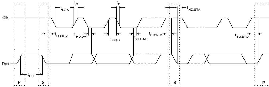
Figure 8.1: Timing Measurements
