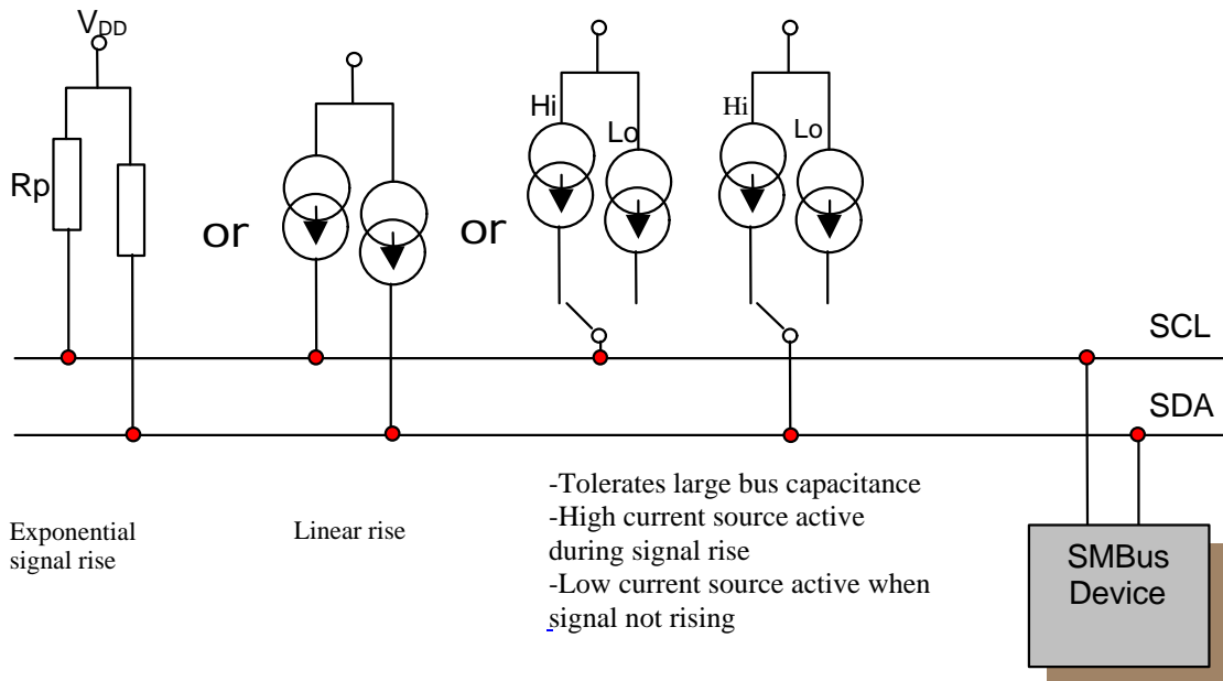
Figure 2.3: SMBus pullup circuitry
