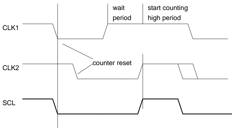
Figure 5.1: SMBus clock synchronization
