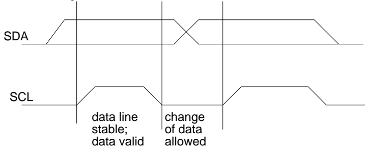
Figure 3.1: Data validity
